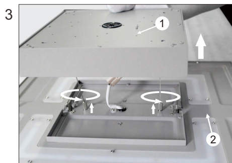
Product list: ① Ceiling box ② lamp body
