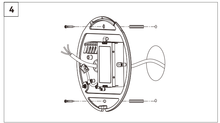
Put AC cable through the hole, and fix the backplate to the wall by 2 screws
