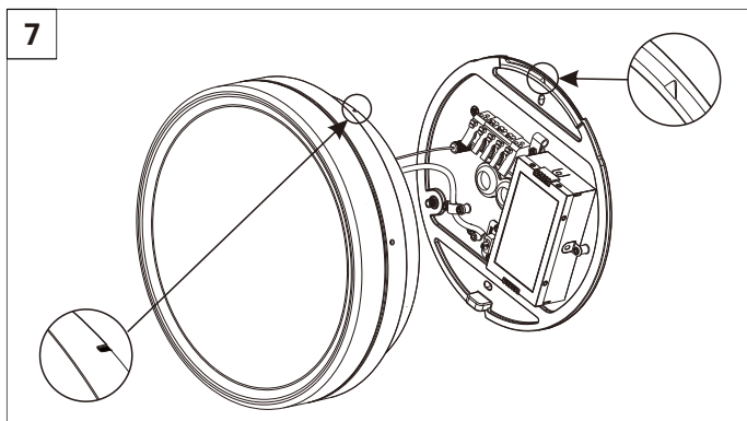
Insert the lamp body into the backplate, please make sure the small notch is aligned with the Arrow mark from backplate.
