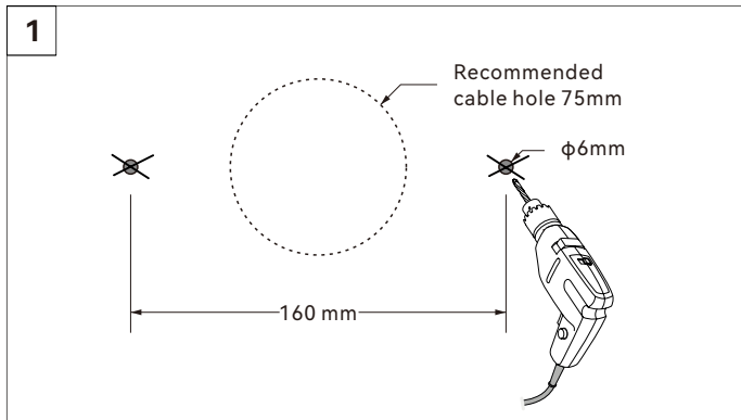
Dimensions of mounting holes
