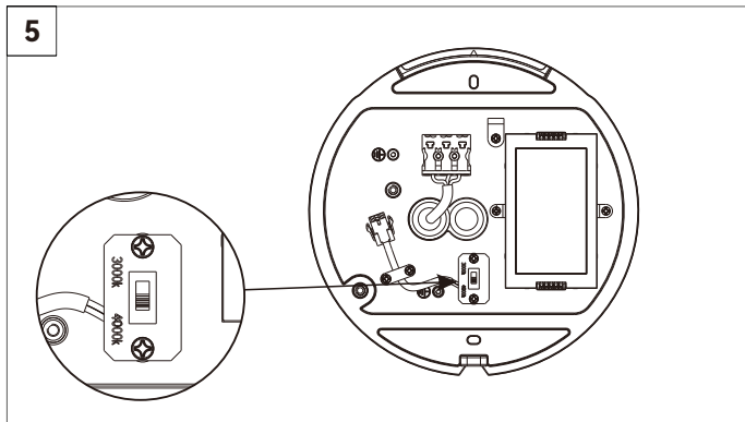
Insert the AC cable to the terminal blocks, and switch the CCT to the request position
