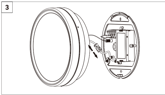
Disconnect the wires and safety steel rope
