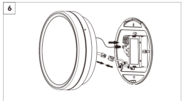
Connect the safety steel rope and wires.
