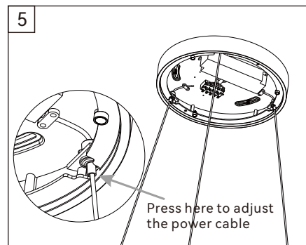
Adjust the length of power cable
