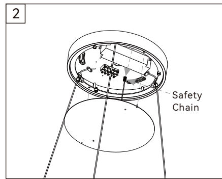
Take off the magnetic front cover
