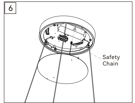
Fix the magnetic front cover onto the driver box housing (Pay attention to aligning the hole position)
