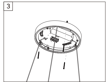
Connector the power cable and fix the driver box onto the ceiling
